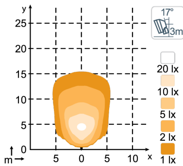
Scorpius GO 410, 1000lm Wide Flood
