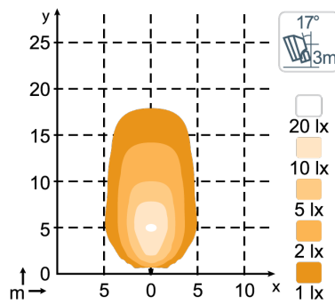
Scorpius GO 410, 1000lm Flood
