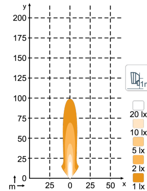
Scorpius GO 410, 1000lm High Beam
